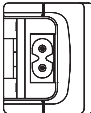
Power Supply connections: Figure 8 line cord input (left), wired positive and negative connections (right).
